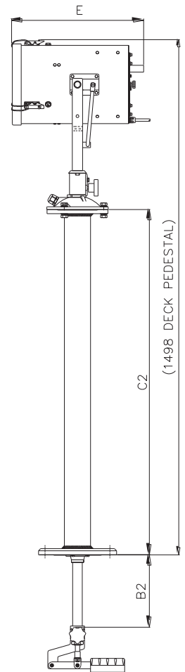
CABIN PEDESTAL CONTROL
